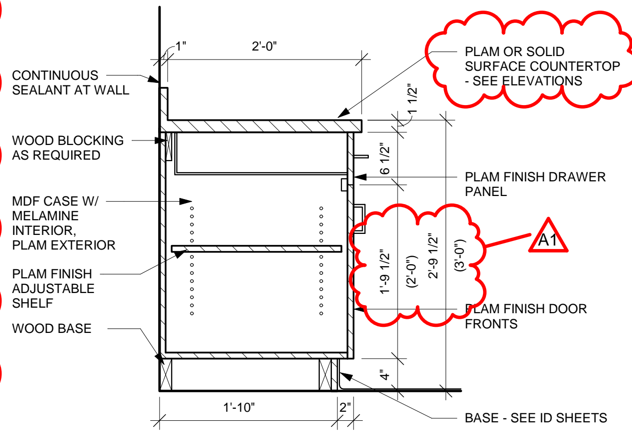
4 CSWK SECTION 1" = 1'-0"
