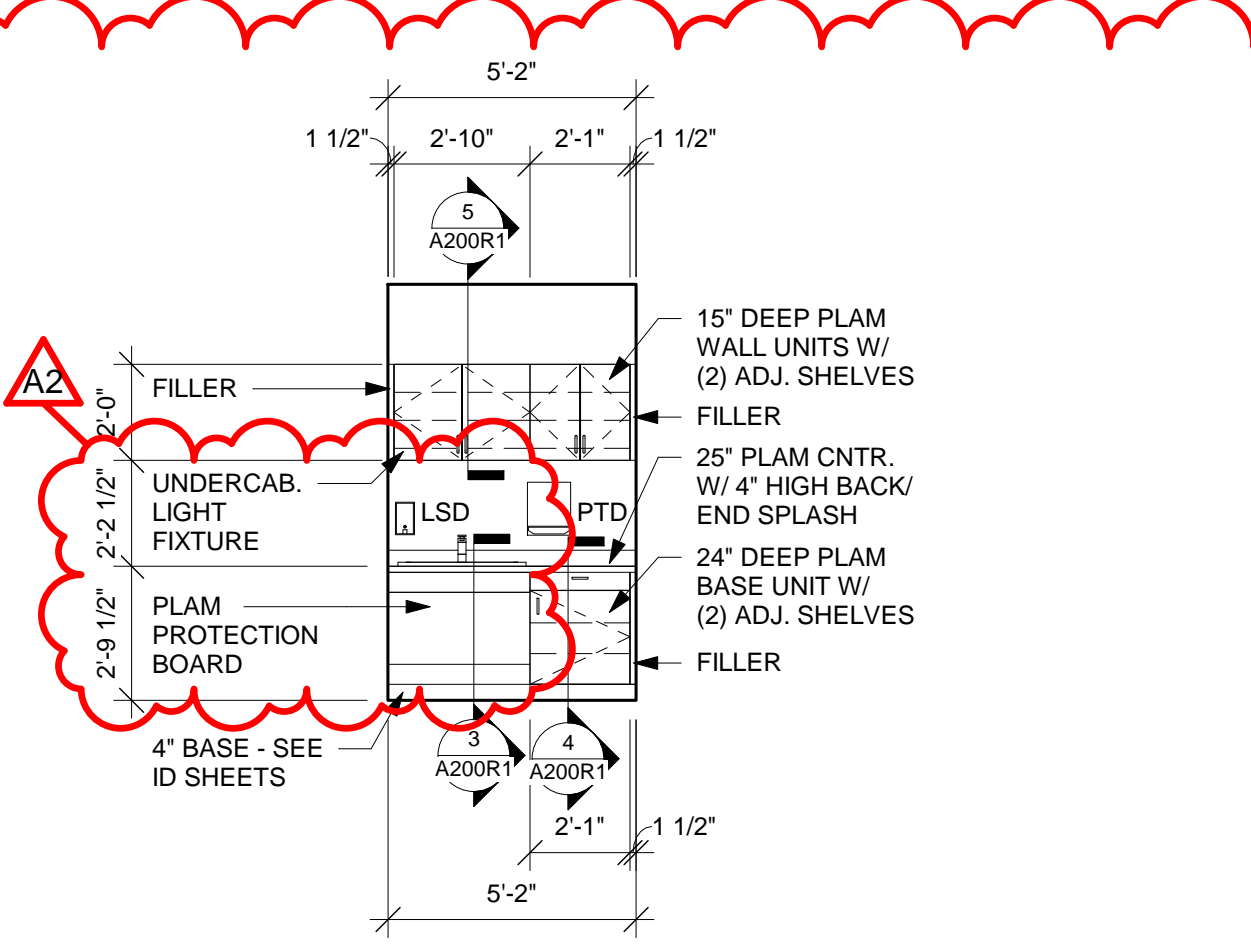
10 CASEWORK ELEV 1/4" = 1'-0"
