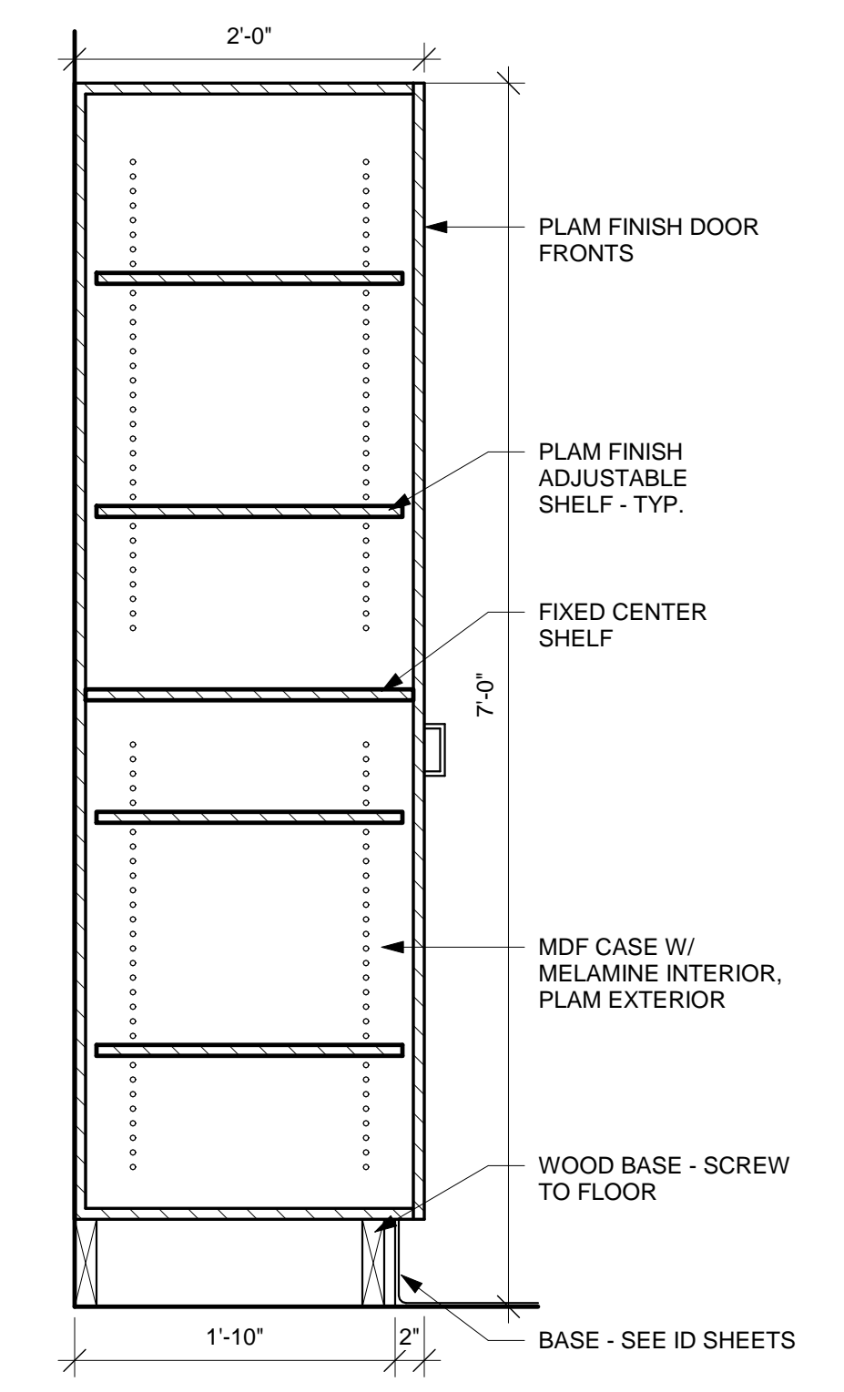
6 CSWK - TALL CAB 1" = 1'-0"
