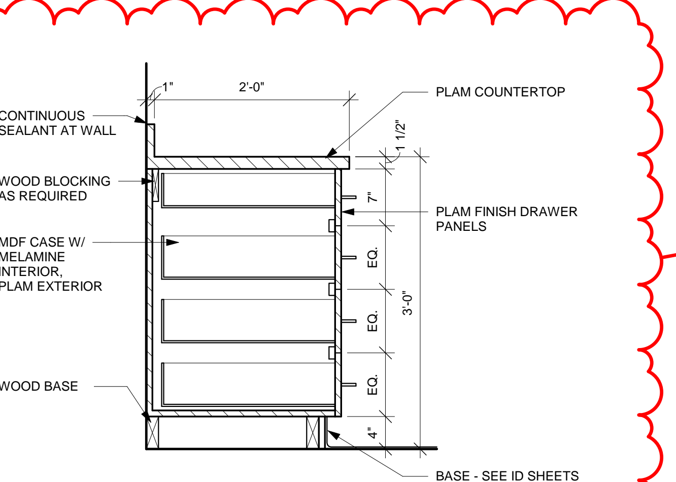
11 CSWK SECTION 1" = 1'-0"
