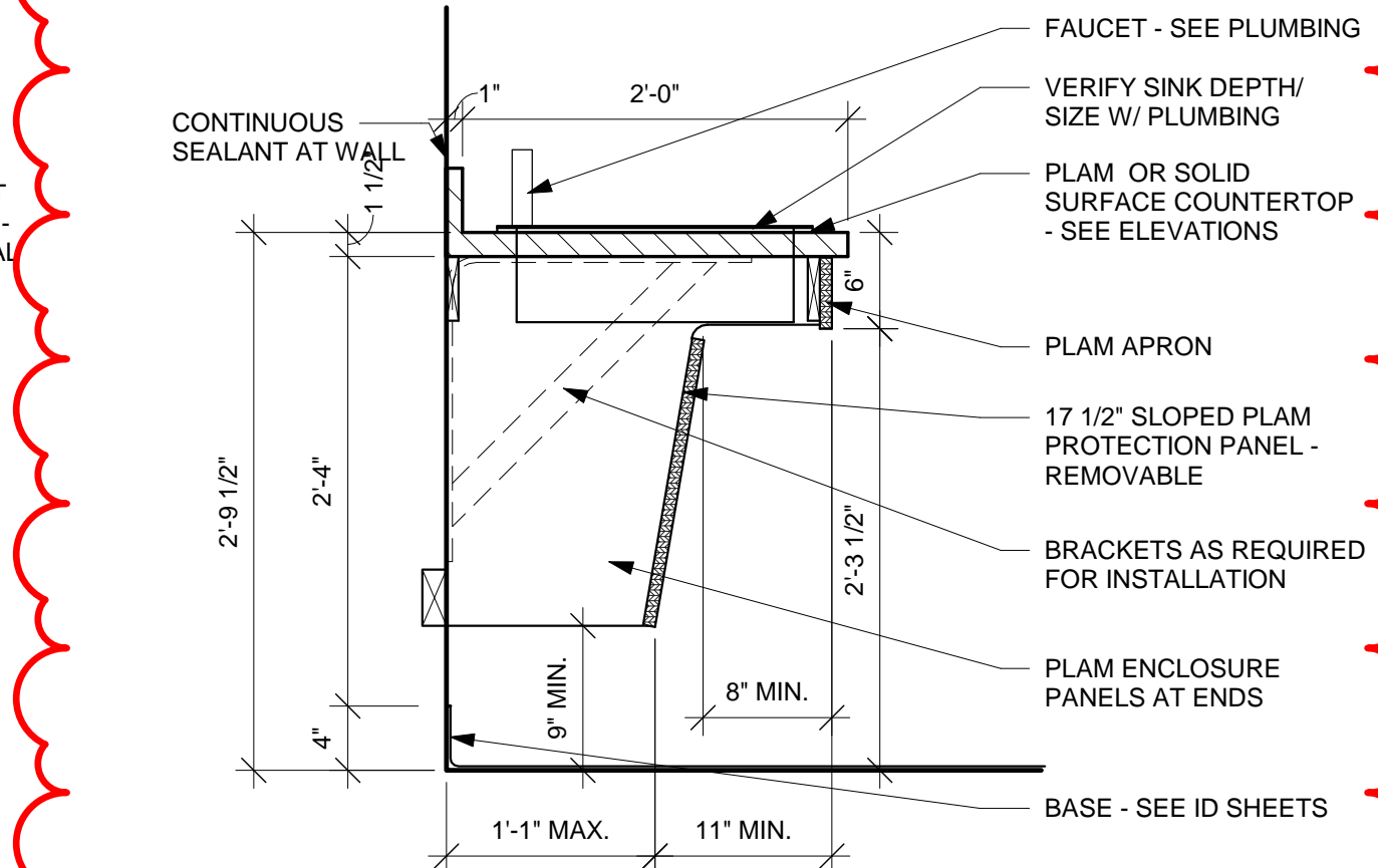
3 CSWK SECTION 1" = 1'-0"
