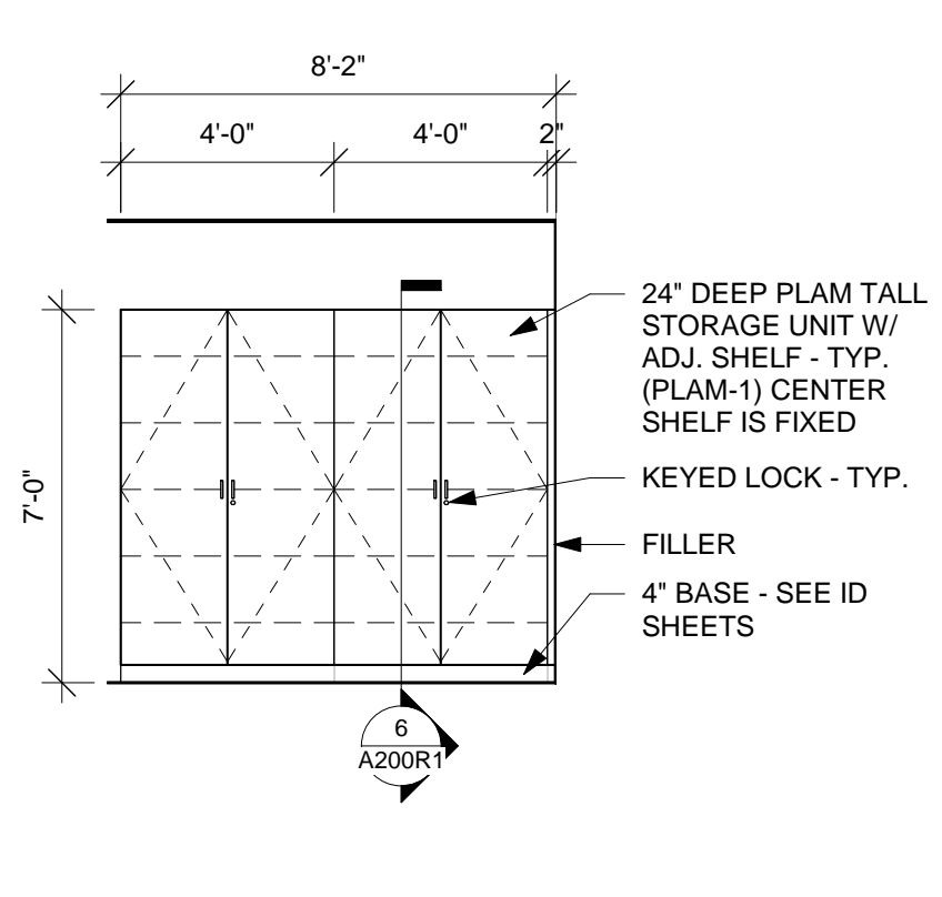
1 CASEWORK ELEV 1/4" = 1'-0"
