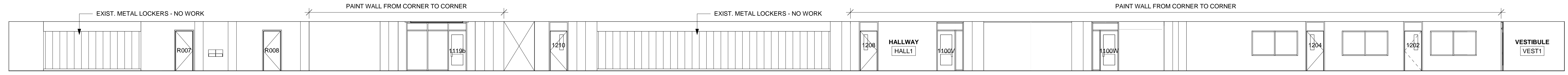
7 INTERIOR ELEVATION 1/8" = 1'-0"
