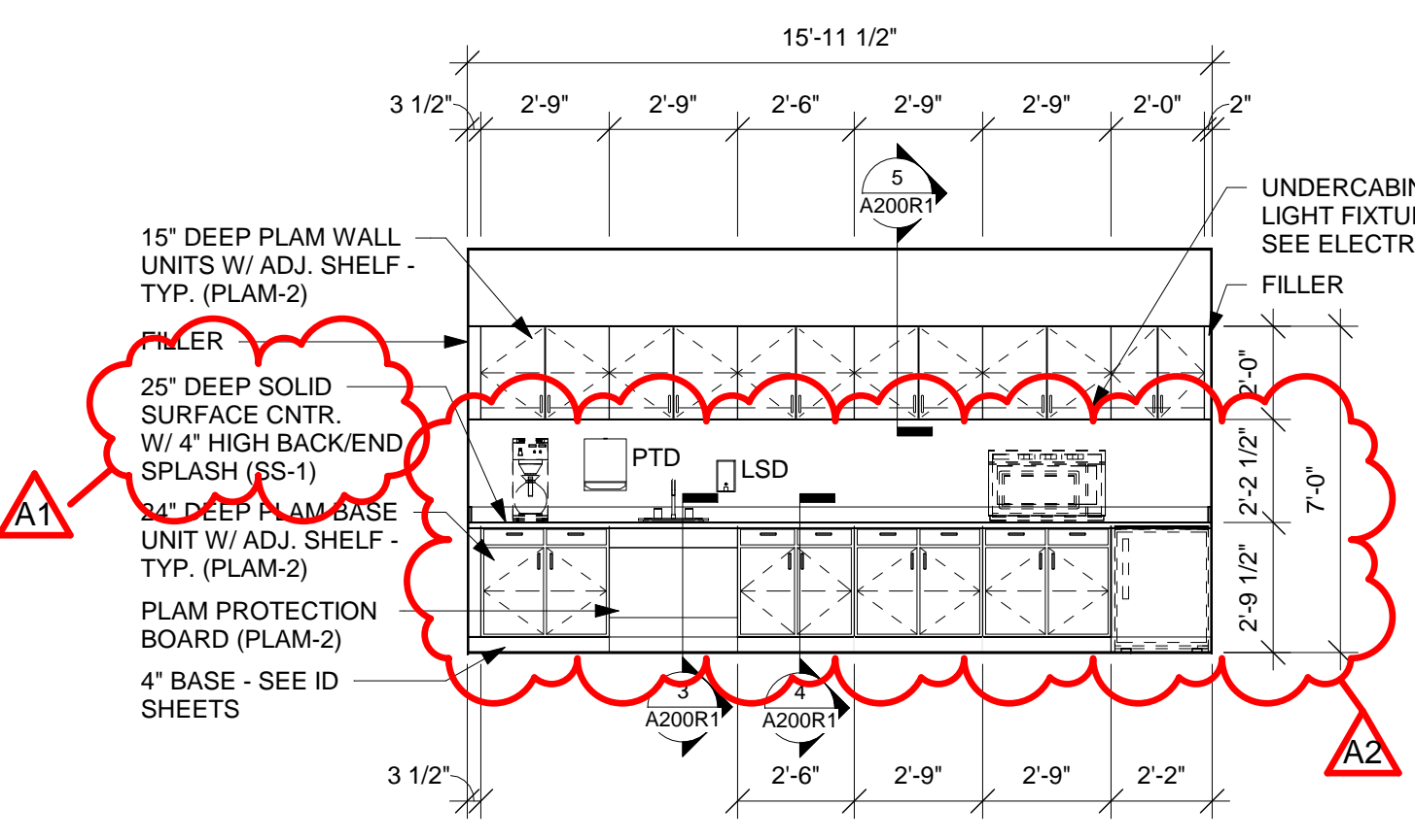
2 CASEWORK ELEV 1/4" = 1'-0"
