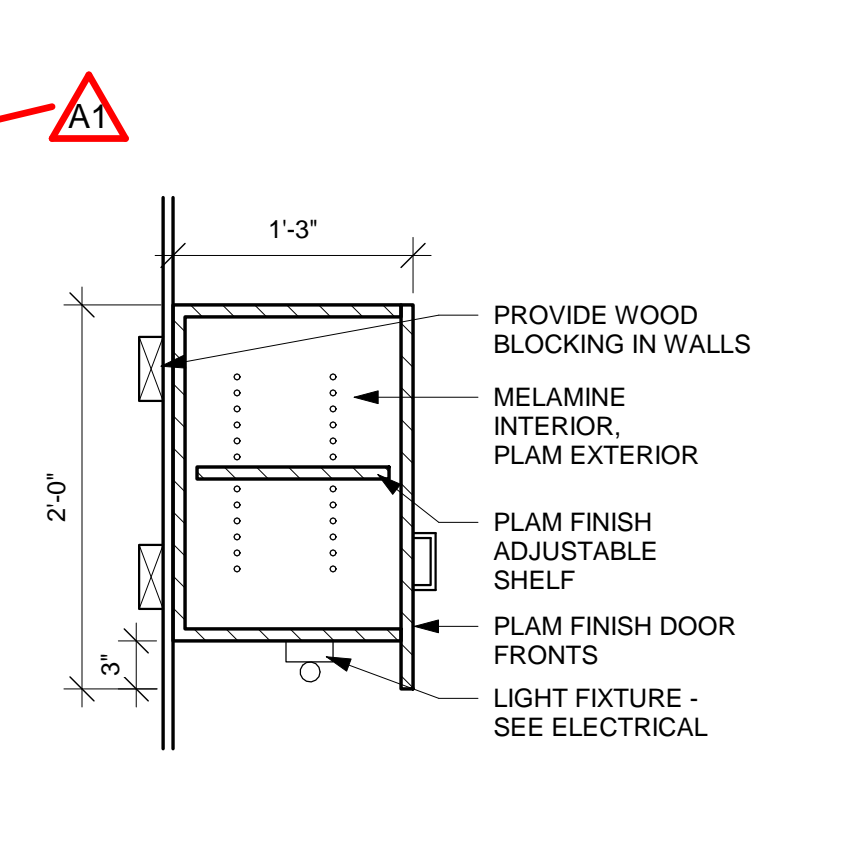
5 CSWK SECTION 1" = 1'-0"
